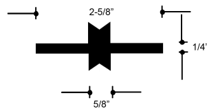
#352-11: 2-5/8"
