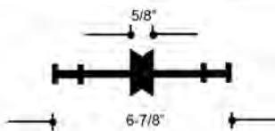
#352-12: 6-7/8"
