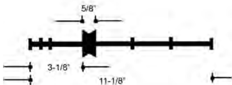
#352-13: 11-1/8"
