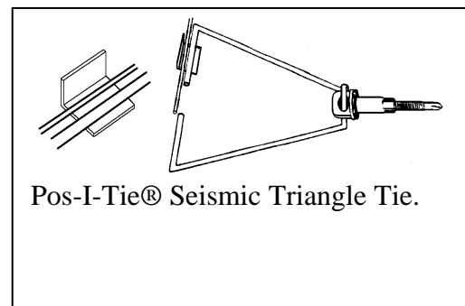
#316 Triangle Tie with Welded #370 Seismic Hook Tab
